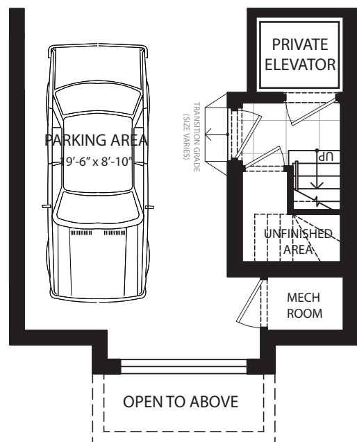
Parking Level
